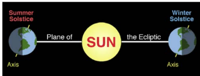
Figure 12. Increased tilt of Earth's spin axis exposes both poles to greater melt of high latitude ice.
