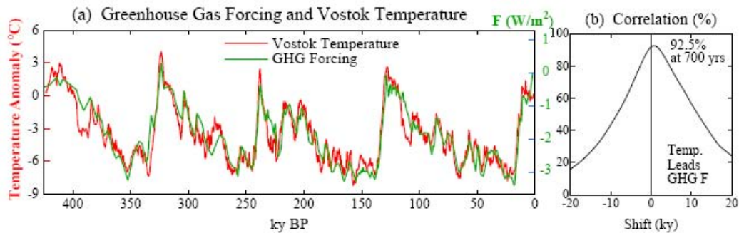
Figure 7. (a) Antarctic temperature from Vostok ice core (Vimeux et al. 2002) and global climate forcing (right scale) due to \text{CO}_2 , \text{CH}_4 and \text{N}_2\text{O} . (b) Correlation (%) diagram showing lead of temperature over greenhouse forcing.
