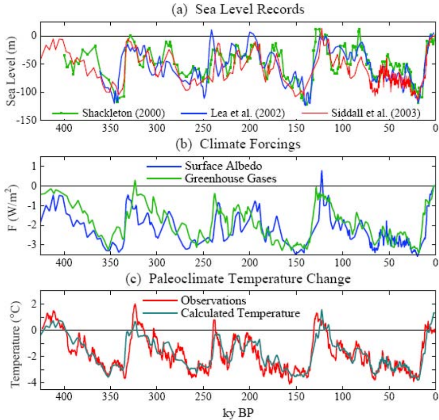
Figure 6. (a) sea level records from three sources, (b) climate forcings due to greenhouse gases ( \text{CO}_2 , \text{CH}_4 and \text{N}_2\text{O} ) and surface albedo from the Siddall et al. sea level record, (c) calculated and observed paleo temperature change. Calculated temperature is the product of the sum of the two forcings in (b) and \frac{3}{4}^\circ\text{C} per \text{W}/\text{m}^2 . Observed temperature is the Vostok temperature (Figure 2) divided by two.
